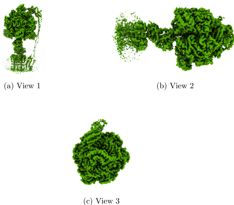
Figure 4: Isosurface at threshold=0.006350. Views generated by ChimeraX at a the following X, Y, Z angles: View 1 (0, -90, -90), View 2 (-90, 0, -90), View 3 (0, 0, 0).
