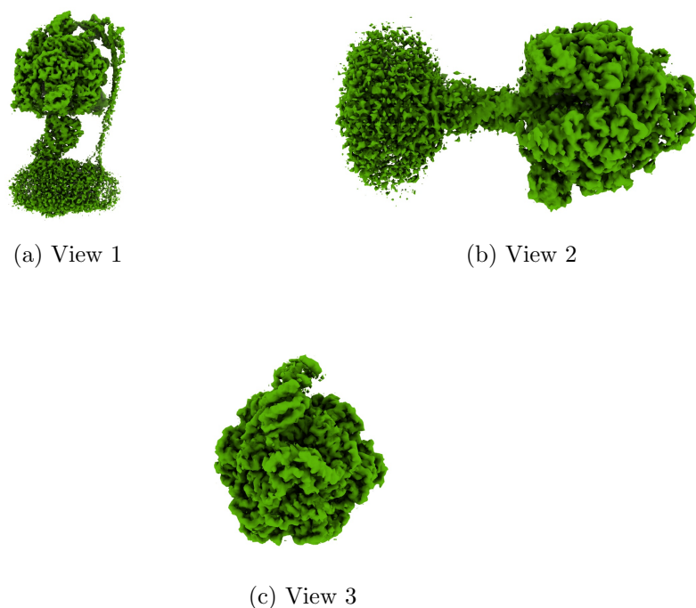
Figure 4: Isosurface at threshold=0.005450. Views generated by ChimeraX at a the following X, Y, Z angles: View 1 (0, -90, -90), View 2 (-90, 0, -90), View 3 (0, 0, 0).
