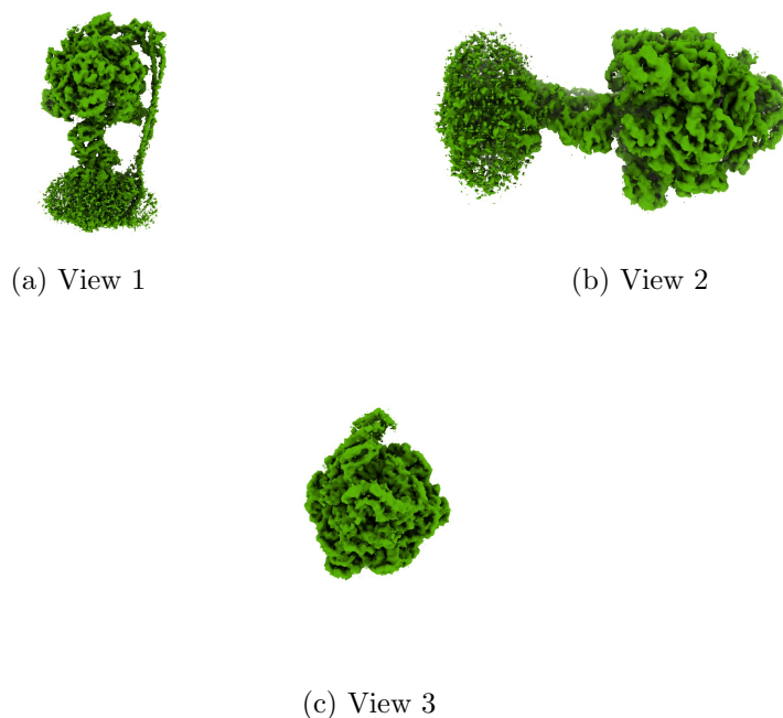
Figure 4: Isosurface at threshold=0.004960. Views generated by ChimeraX at a the following X, Y, Z angles: View 1 (0, -90, -90), View 2 (-90, 0, -90), View 3 (0, 0, 0).
