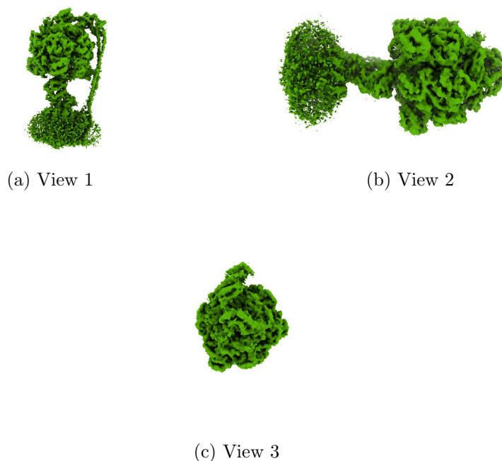
Figure 4: Isosurface at threshold=0.004930. Views generated by ChimeraX at a the following X, Y, Z angles: View 1 (0, -90, -90), View 2 (-90, 0, -90), View 3 (0, 0, 0).
