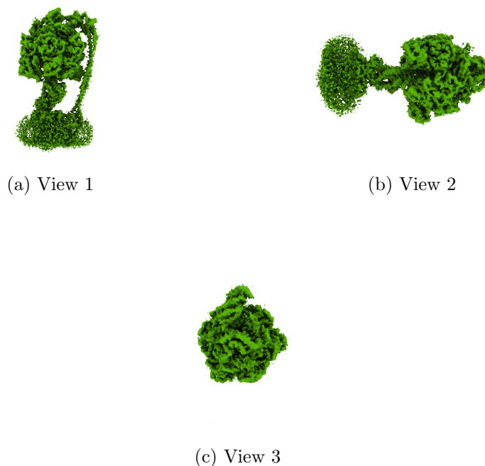
Figure 4: Isosurface at threshold=0.004960. Views generated by ChimeraX at a the following X, Y, Z angles: View 1 (0, -90, -90), View 2 (-90, 0, -90), View 3 (0, 0, 0).
