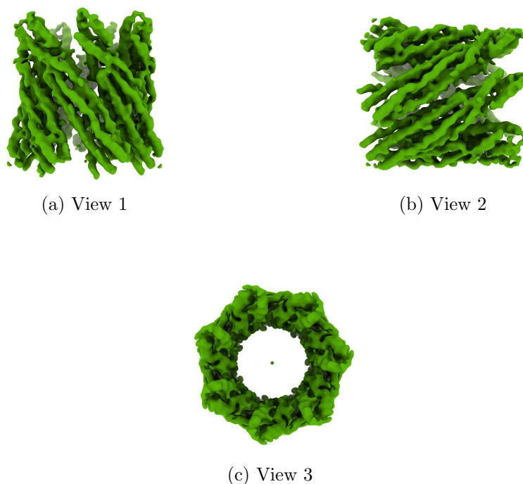
Figure 4: Isosurface at threshold=0.013700. Views generated by ChimeraX at a the following X, Y, Z angles: View 1 (0, -90, -90), View 2 (-90, 0, -90), View 3 (0, 0, 0).
