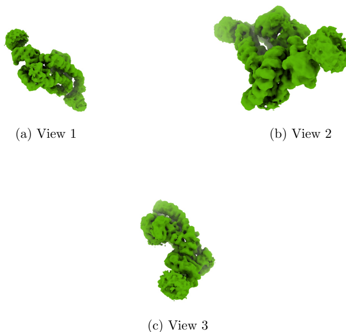
Figure 4: Isosurface at threshold=0.003700. Views generated by ChimeraX at a the following X, Y, Z angles: View 1 (0, -90, -90), View 2 (-90, 0, -90), View 3 (0, 0, 0).
