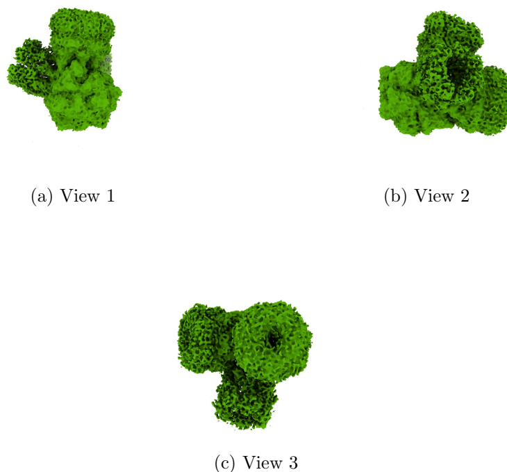
Figure 4: Isosurface at threshold=0.003800. Views generated by ChimeraX at a the following X, Y, Z angles: View 1 (0, -90, -90), View 2 (-90, 0, -90), View 3 (0, 0, 0).
