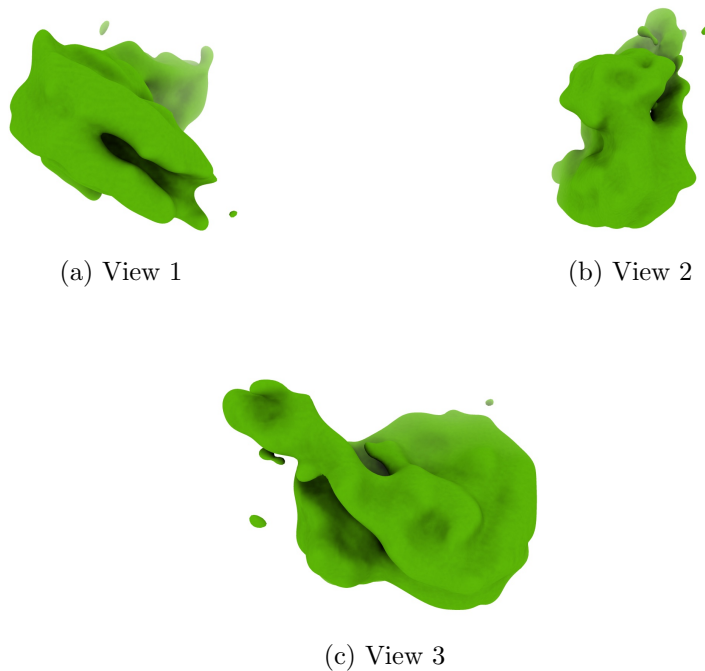
Figure 4: Isosurface at threshold=0.049000. Views generated by ChimeraX at a the following X, Y, Z angles: View 1 (0, -90, -90), View 2 (-90, 0, -90), View 3 (0, 0, 0).
