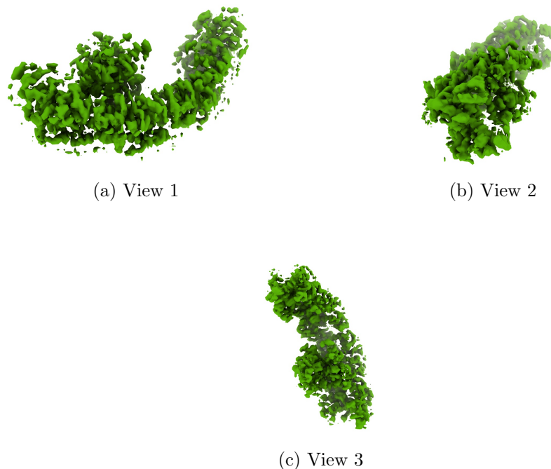
Figure 4: Isosurface at threshold=0.318000. Views generated by ChimeraX at a the following X, Y, Z angles: View 1 (0, -90, -90), View 2 (-90, 0, -90), View 3 (0, 0, 0).
