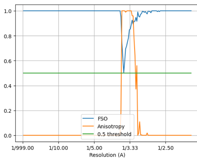
Figure 32: FSO and anisotropy.
