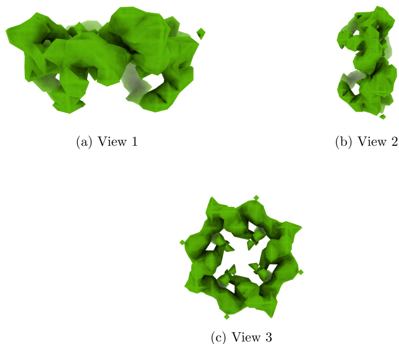
Figure 4: Isosurface at threshold=0.010100. Views generated by ChimeraX at a the following X, Y, Z angles: View 1 (0, -90, -90), View 2 (-90, 0, -90), View 3 (0, 0, 0).
