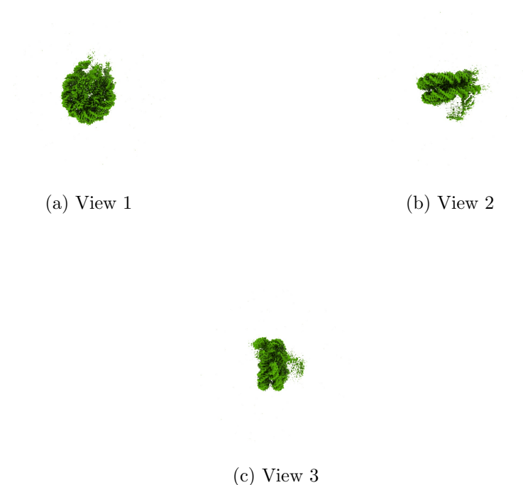
Figure 4: Isosurface at threshold=0.259000. Views generated by ChimeraX at a the following X, Y, Z angles: View 1 (0, -90, -90), View 2 (-90, 0, -90), View 3 (0, 0, 0).
