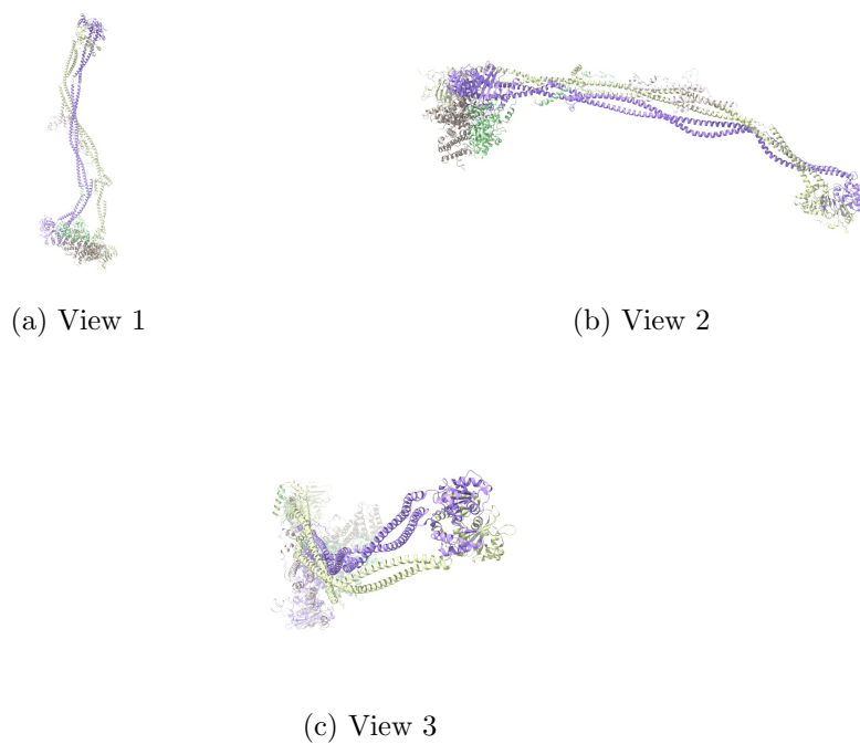
Figure 10: Input atomic model Views generated by ChimeraX at the following X, Y, Z angles: View 1 (0, -90, -90), View 2 (-90, 0, -90), View 3 (0, 0, 0).
