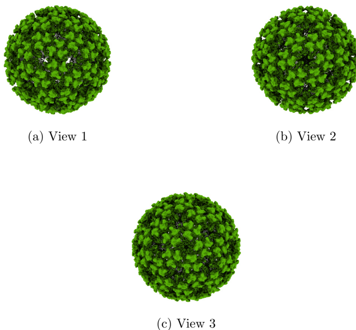
Figure 4: Isosurface at threshold=0.007500. Views generated by ChimeraX at a the following X, Y, Z angles: View 1 (0, -90, -90), View 2 (-90, 0, -90), View 3 (0, 0, 0).
