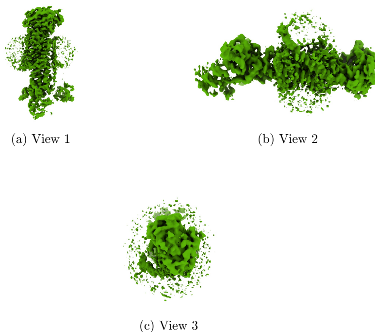
Figure 4: Isosurface at threshold=0.218000. Views generated by ChimeraX at a the following X, Y, Z angles: View 1 (0, -90, -90), View 2 (-90, 0, -90), View 3 (0, 0, 0).
