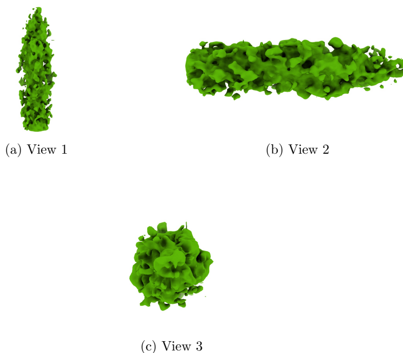
Figure 4: Isosurface at threshold=0.788000. Views generated by ChimeraX at a the following X, Y, Z angles: View 1 (0, -90, -90), View 2 (-90, 0, -90), View 3 (0, 0, 0).
