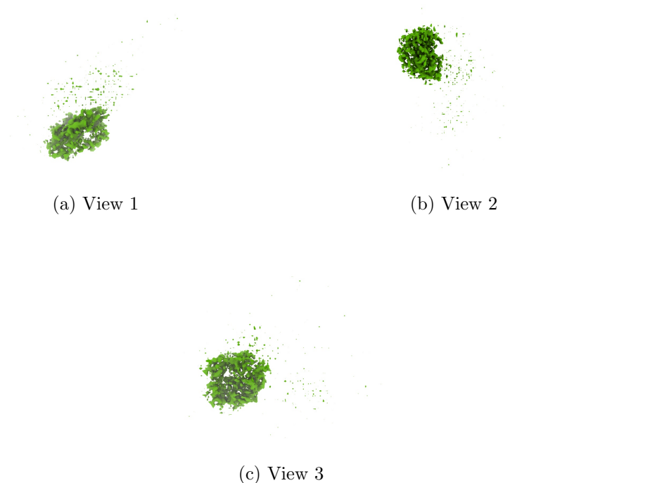
Figure 4: Isosurface at threshold=0.550000. Views generated by ChimeraX at a the following X, Y, Z angles: View 1 (0, -90, -90), View 2 (-90, 0, -90), View 3 (0, 0, 0).
