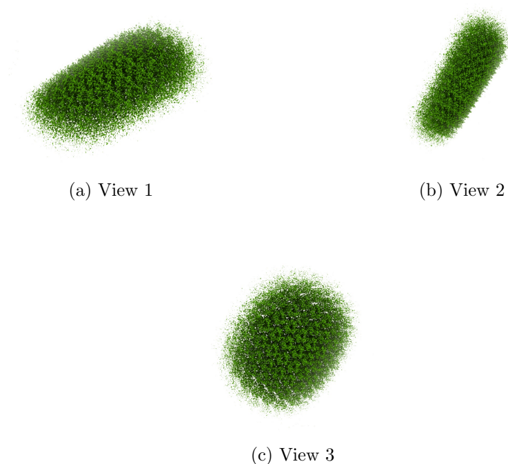
Figure 4: Isosurface at threshold=3.700000. Views generated by ChimeraX at a the following X, Y, Z angles: View 1 (0, -90, -90), View 2 (-90, 0, -90), View 3 (0, 0, 0).
