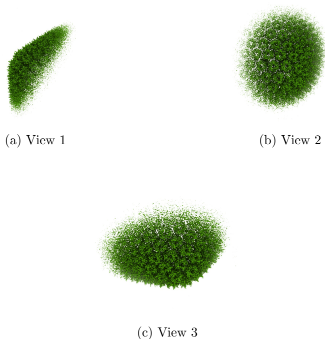
Figure 4: Isosurface at threshold=3.700000. Views generated by ChimeraX at a the following X, Y, Z angles: View 1 (0, -90, -90), View 2 (-90, 0, -90), View 3 (0, 0, 0).
