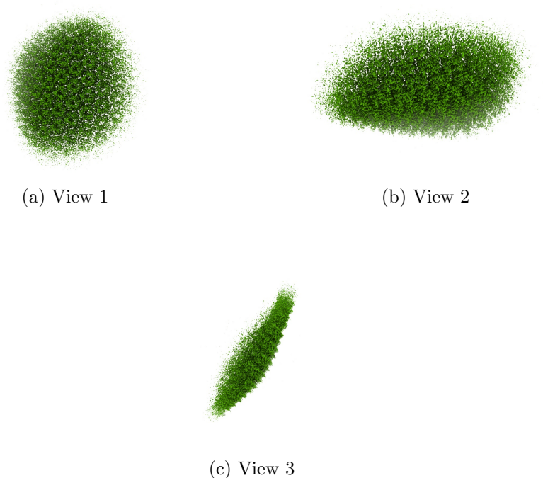
Figure 4: Isosurface at threshold=3.700000. Views generated by ChimeraX at a the following X, Y, Z angles: View 1 (0, -90, -90), View 2 (-90, 0, -90), View 3 (0, 0, 0).
