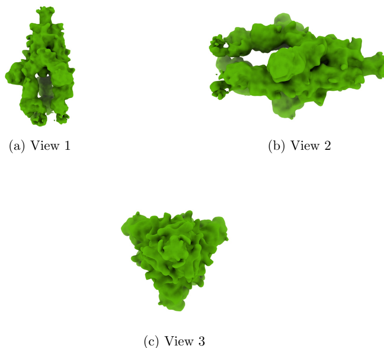
Figure 4: Isosurface at threshold=0.269000. Views generated by ChimeraX at a the following X, Y, Z angles: View 1 (0, -90, -90), View 2 (-90, 0, -90), View 3 (0, 0, 0).
