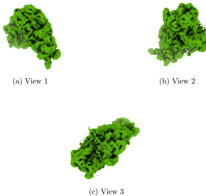
Figure 4: Isosurface at threshold=0.024500. Views generated by ChimeraX at a the following X, Y, Z angles: View 1 (0, -90, -90), View 2 (-90, 0, -90), View 3 (0, 0, 0).
