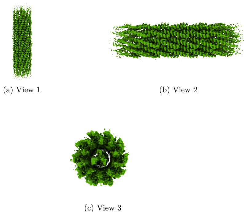
Figure 4: Isosurface at threshold=0.019100. Views generated by ChimeraX at a the following X, Y, Z angles: View 1 (0, -90, -90), View 2 (-90, 0, -90), View 3 (0, 0, 0).
