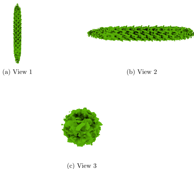
Figure 4: Isosurface at threshold=0.004400. Views generated by ChimeraX at a the following X, Y, Z angles: View 1 (0, -90, -90), View 2 (-90, 0, -90), View 3 (0, 0, 0).
