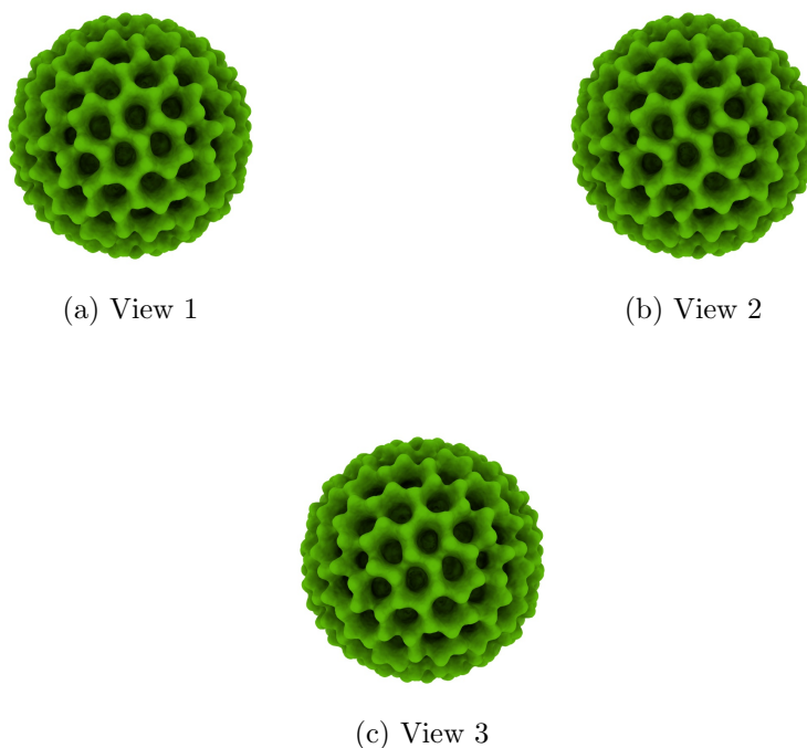
Figure 4: Isosurface at threshold=0.657000. Views generated by ChimeraX at a the following X, Y, Z angles: View 1 (0, -90, -90), View 2 (-90, 0, -90), View 3 (0, 0, 0).
