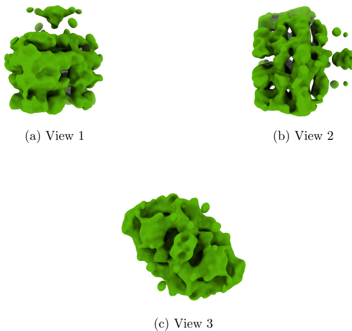
Figure 4: Isosurface at threshold=1.390000. Views generated by ChimeraX at a the following X, Y, Z angles: View 1 (0, -90, -90), View 2 (-90, 0, -90), View 3 (0, 0, 0).
