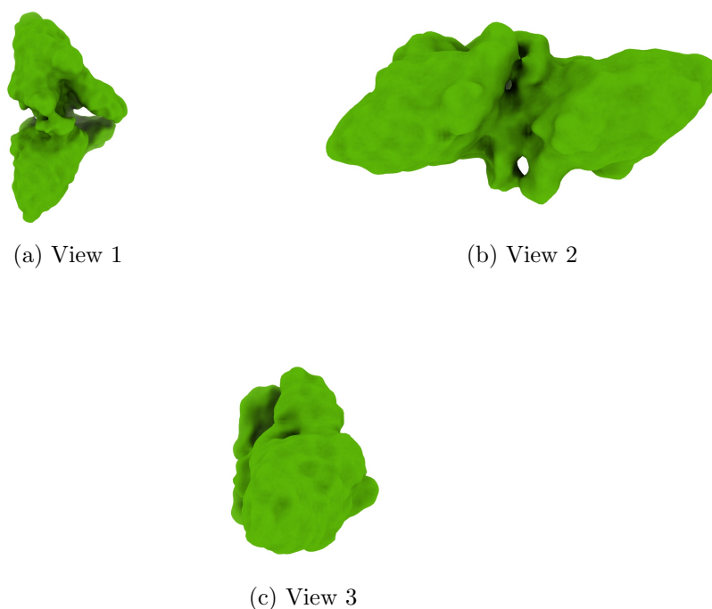
Figure 4: Isosurface at threshold=0.734000. Views generated by ChimeraX at a the following X, Y, Z angles: View 1 (0, -90, -90), View 2 (-90, 0, -90), View 3 (0, 0, 0).
