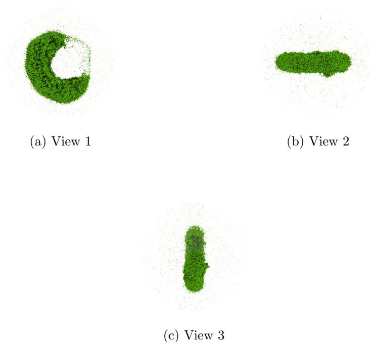
Figure 4: Isosurface at threshold=0.221000. Views generated by ChimeraX at a the following X, Y, Z angles: View 1 (0, -90, -90), View 2 (-90, 0, -90), View 3 (0, 0, 0).
