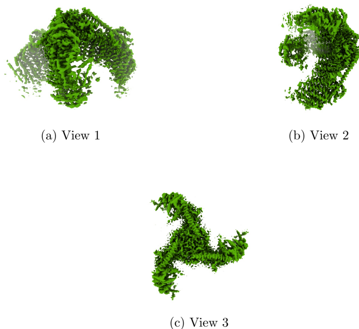
Figure 4: Isosurface at threshold=0.763000. Views generated by ChimeraX at a the following X, Y, Z angles: View 1 (0, -90, -90), View 2 (-90, 0, -90), View 3 (0, 0, 0).
