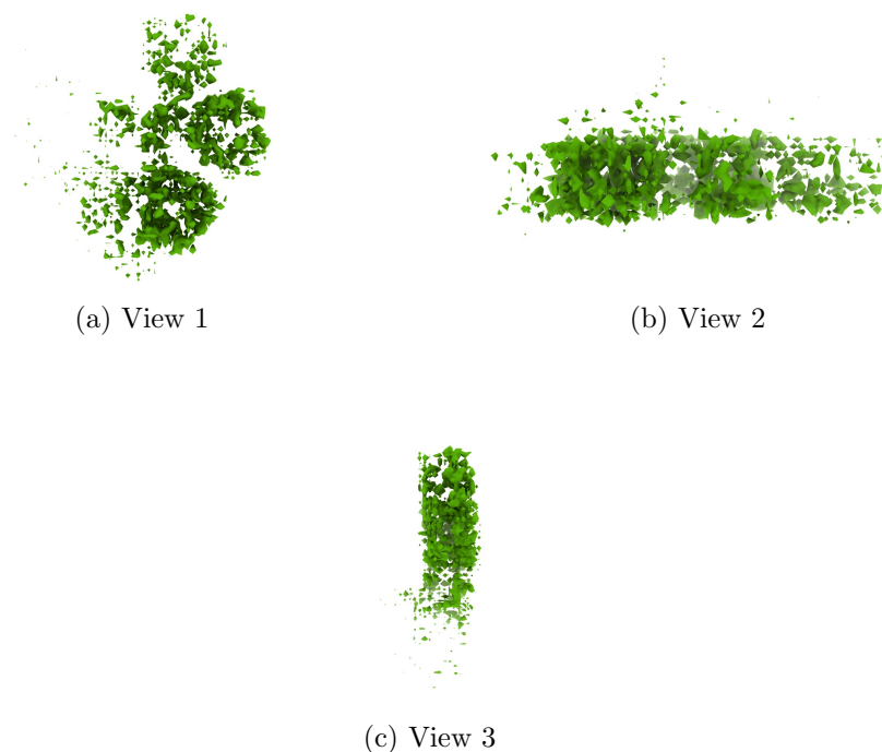
Figure 4: Isosurface at threshold=0.748000. Views generated by ChimeraX at a the following X, Y, Z angles: View 1 (0, -90, -90), View 2 (-90, 0, -90), View 3 (0, 0, 0).
