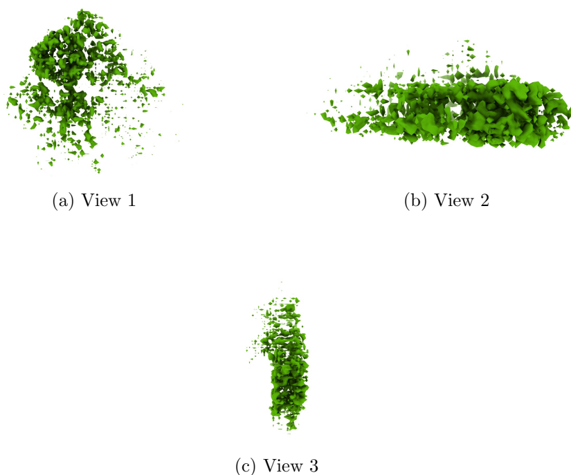
Figure 4: Isosurface at threshold=0.535000. Views generated by ChimeraX at a the following X, Y, Z angles: View 1 (0, -90, -90), View 2 (-90, 0, -90), View 3 (0, 0, 0).
