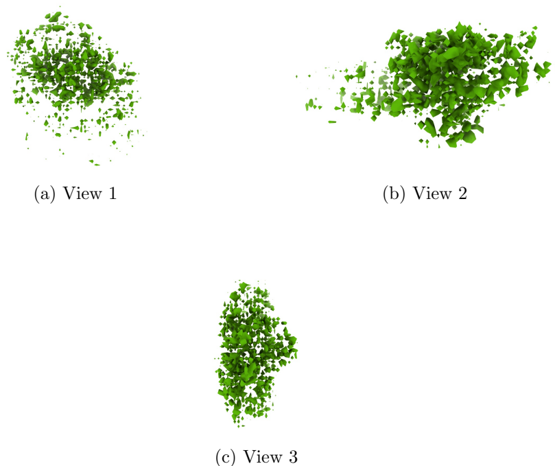
Figure 4: Isosurface at threshold=1.410000. Views generated by ChimeraX at a the following X, Y, Z angles: View 1 (0, -90, -90), View 2 (-90, 0, -90), View 3 (0, 0, 0).
