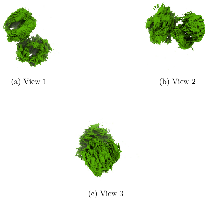
Figure 4: Isosurface at threshold=0.076000. Views generated by ChimeraX at a the following X, Y, Z angles: View 1 (0, -90, -90), View 2 (-90, 0, -90), View 3 (0, 0, 0).
