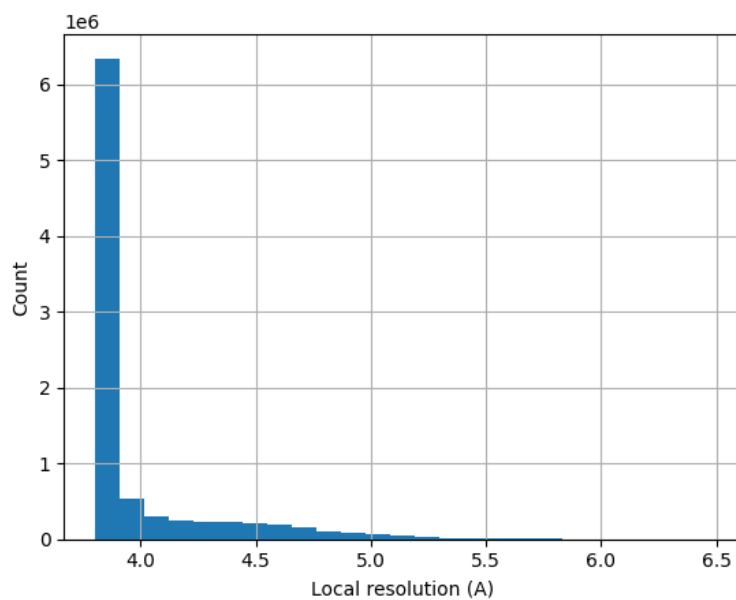
Figure 23: Histogram of the local resolution according to Resmap.
