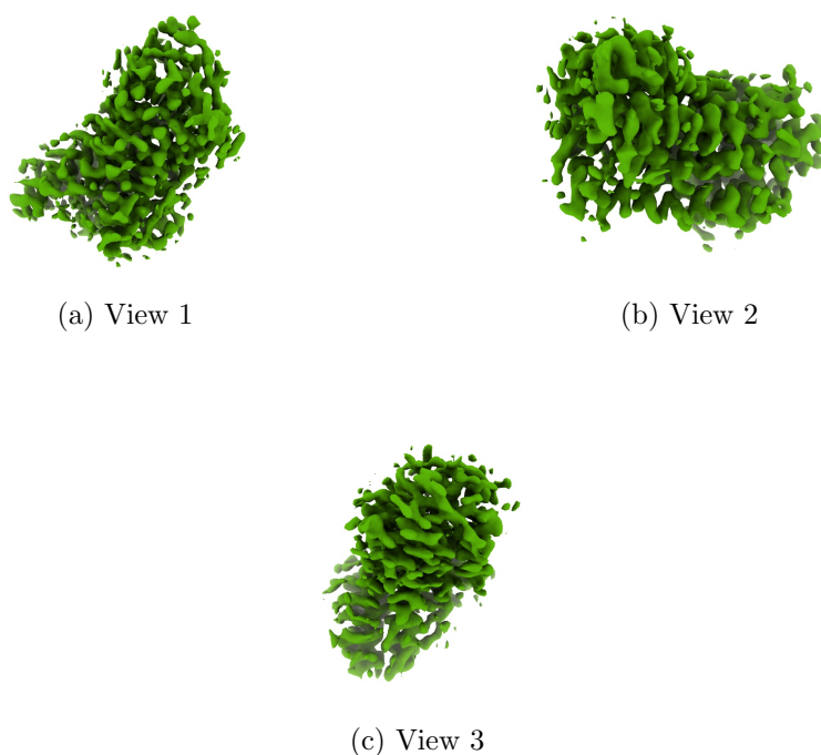
Figure 4: Isosurface at threshold=0.678000. Views generated by ChimeraX at a the following X, Y, Z angles: View 1 (0, -90, -90), View 2 (-90, 0, -90), View 3 (0, 0, 0).
