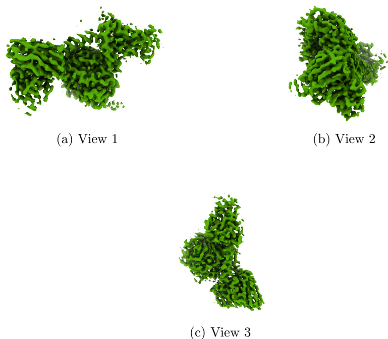
Figure 4: Isosurface at threshold=0.828000. Views generated by ChimeraX at a the following X, Y, Z angles: View 1 (0, -90, -90), View 2 (-90, 0, -90), View 3 (0, 0, 0).
