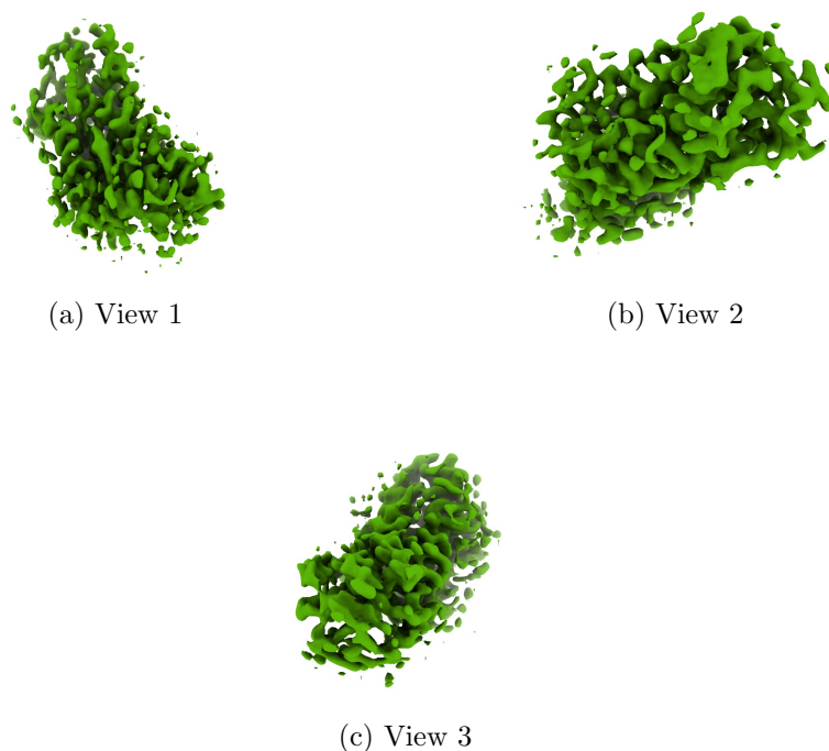
Figure 4: Isosurface at threshold=0.511000. Views generated by ChimeraX at a the following X, Y, Z angles: View 1 (0, -90, -90), View 2 (-90, 0, -90), View 3 (0, 0, 0).
