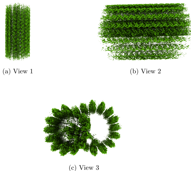
Figure 4: Isosurface at threshold=0.485000. Views generated by ChimeraX at a the following X, Y, Z angles: View 1 (0, -90, -90), View 2 (-90, 0, -90), View 3 (0, 0, 0).
