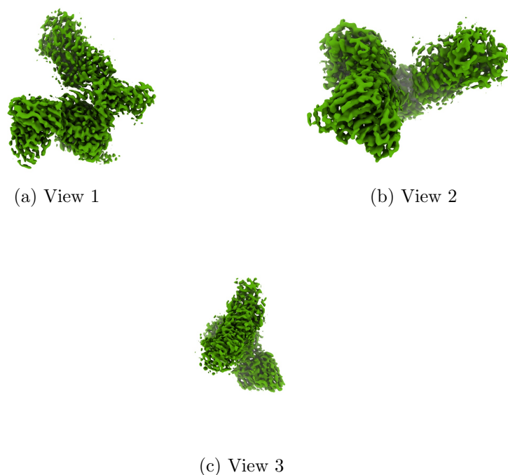
Figure 4: Isosurface at threshold=0.615000. Views generated by ChimeraX at a the following X, Y, Z angles: View 1 (0, -90, -90), View 2 (-90, 0, -90), View 3 (0, 0, 0).
