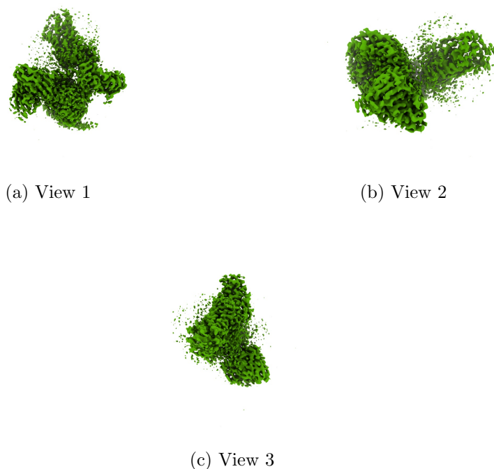
Figure 4: Isosurface at threshold=0.368000. Views generated by ChimeraX at a the following X, Y, Z angles: View 1 (0, -90, -90), View 2 (-90, 0, -90), View 3 (0, 0, 0).
