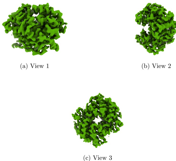
Figure 4: Isosurface at threshold=0.070100. Views generated by ChimeraX at a the following X, Y, Z angles: View 1 (0, -90, -90), View 2 (-90, 0, -90), View 3 (0, 0, 0).
