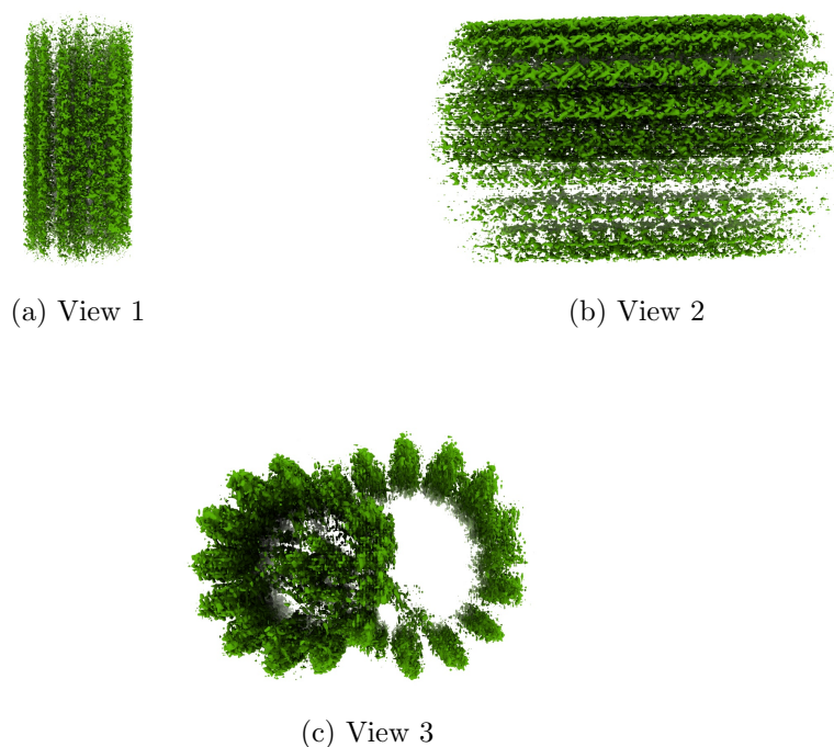
Figure 4: Isosurface at threshold=0.429000. Views generated by ChimeraX at a the following X, Y, Z angles: View 1 (0, -90, -90), View 2 (-90, 0, -90), View 3 (0, 0, 0).
