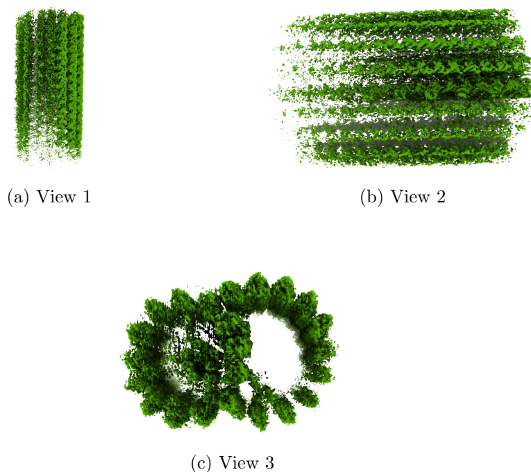
Figure 4: Isosurface at threshold=0.367000. Views generated by ChimeraX at a the following X, Y, Z angles: View 1 (0, -90, -90), View 2 (-90, 0, -90), View 3 (0, 0, 0).
