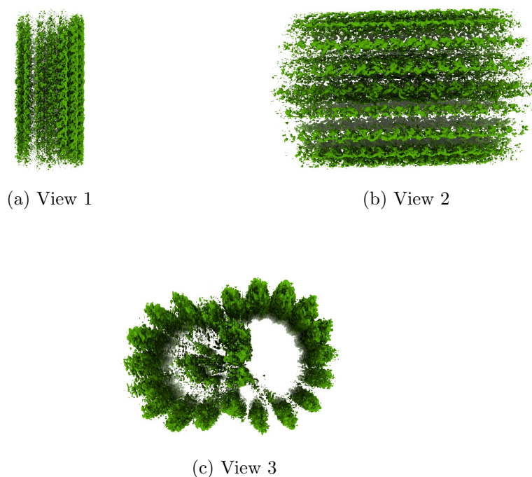
Figure 4: Isosurface at threshold=0.387000. Views generated by ChimeraX at a the following X, Y, Z angles: View 1 (0, -90, -90), View 2 (-90, 0, -90), View 3 (0, 0, 0).
