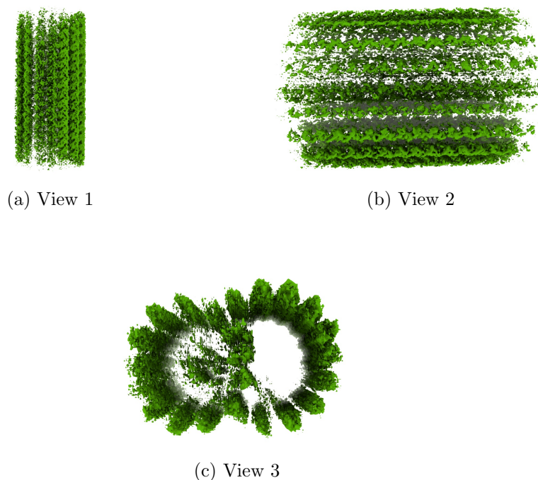
Figure 4: Isosurface at threshold=0.361000. Views generated by ChimeraX at a the following X, Y, Z angles: View 1 (0, -90, -90), View 2 (-90, 0, -90), View 3 (0, 0, 0).
