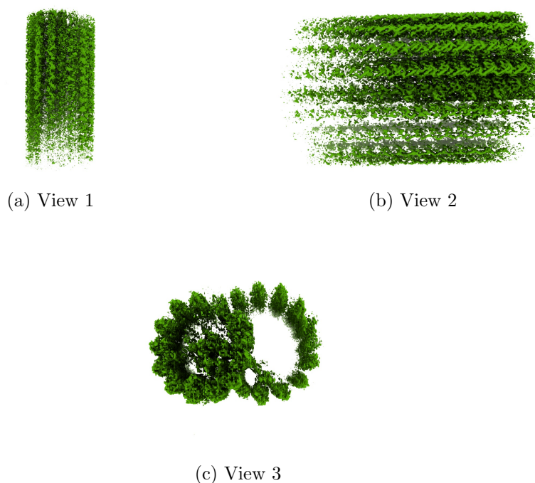
Figure 4: Isosurface at threshold=0.408000. Views generated by ChimeraX at a the following X, Y, Z angles: View 1 (0, -90, -90), View 2 (-90, 0, -90), View 3 (0, 0, 0).
