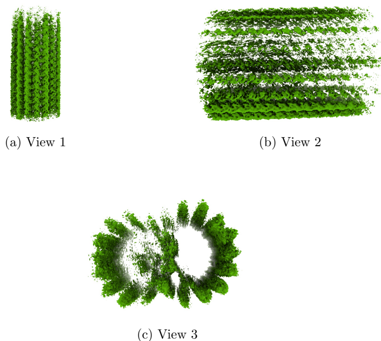
Figure 4: Isosurface at threshold=0.315000. Views generated by ChimeraX at a the following X, Y, Z angles: View 1 (0, -90, -90), View 2 (-90, 0, -90), View 3 (0, 0, 0).
