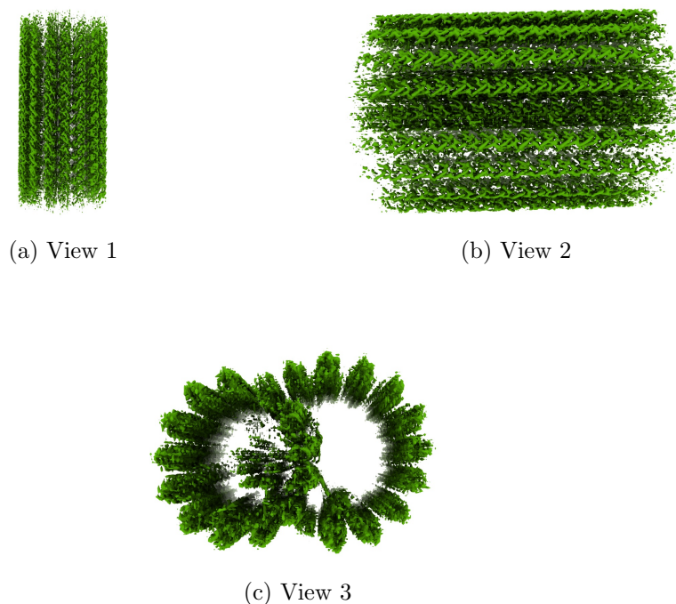
Figure 4: Isosurface at threshold=0.462000. Views generated by ChimeraX at a the following X, Y, Z angles: View 1 (0, -90, -90), View 2 (-90, 0, -90), View 3 (0, 0, 0).
