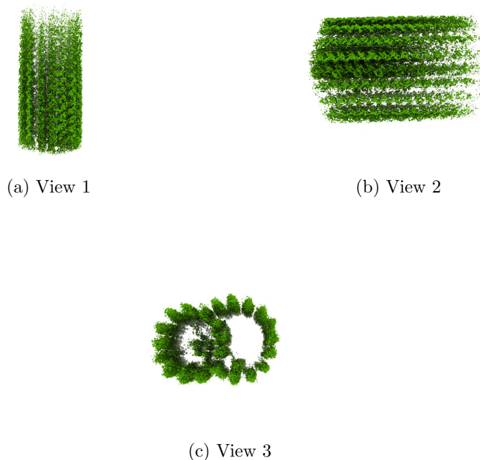
Figure 4: Isosurface at threshold=0.398000. Views generated by ChimeraX at a the following X, Y, Z angles: View 1 (0, -90, -90), View 2 (-90, 0, -90), View 3 (0, 0, 0).
